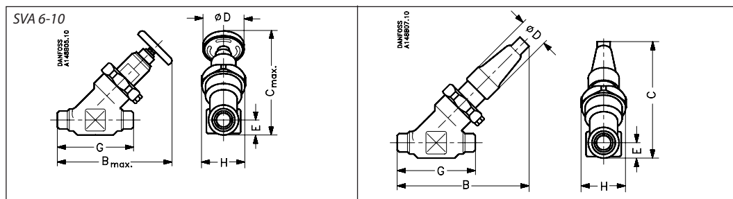
SVA 6 - 10 in straight-way execution with handwheel
